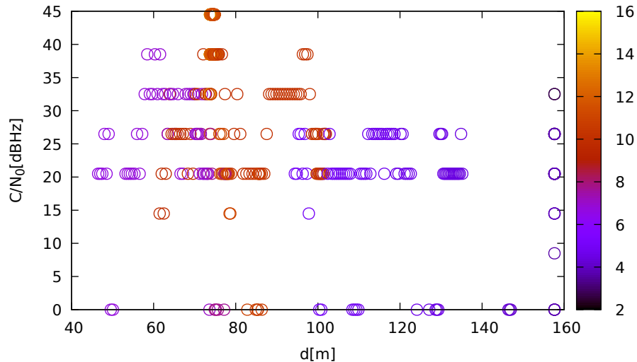
C/N 0 vs distance (LeicaGS18 at C 2 for G27 at L2)
