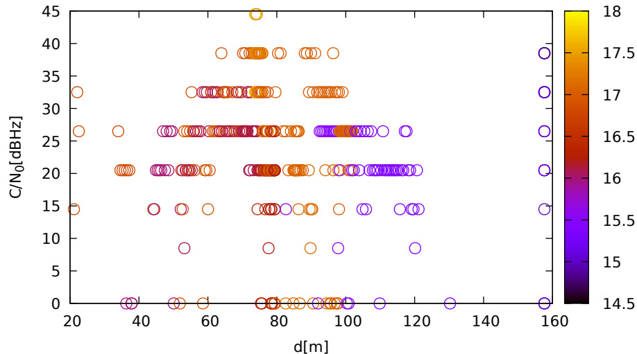
C/N 0 vs distance (LeicaGS18 at C 2 for G28 at L2)
