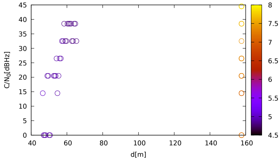
C/N 0 vs distance (LeicaGS18 at C 2 for G31 at L2)
