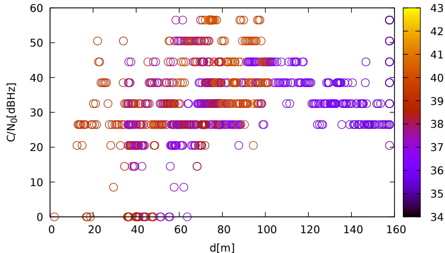
C/N 0 vs distance (LeicaGS18 at C 2 for G32 at L2)
