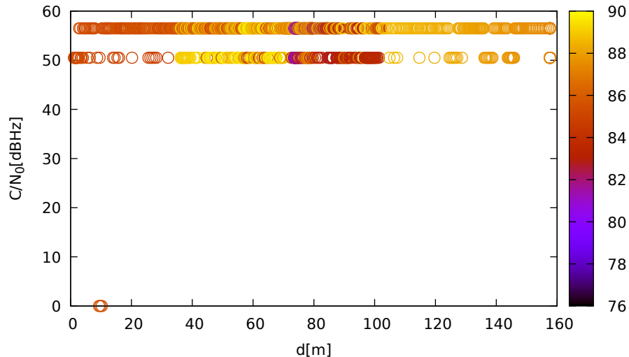
C/N 0 vs distance (LeicaGS18 at C 2 for R07 at L2)
