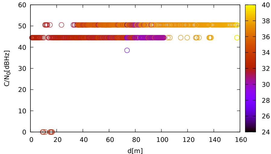
C/N 0 vs distance (LeicaGS18 at C 2 for R08 at L2)
