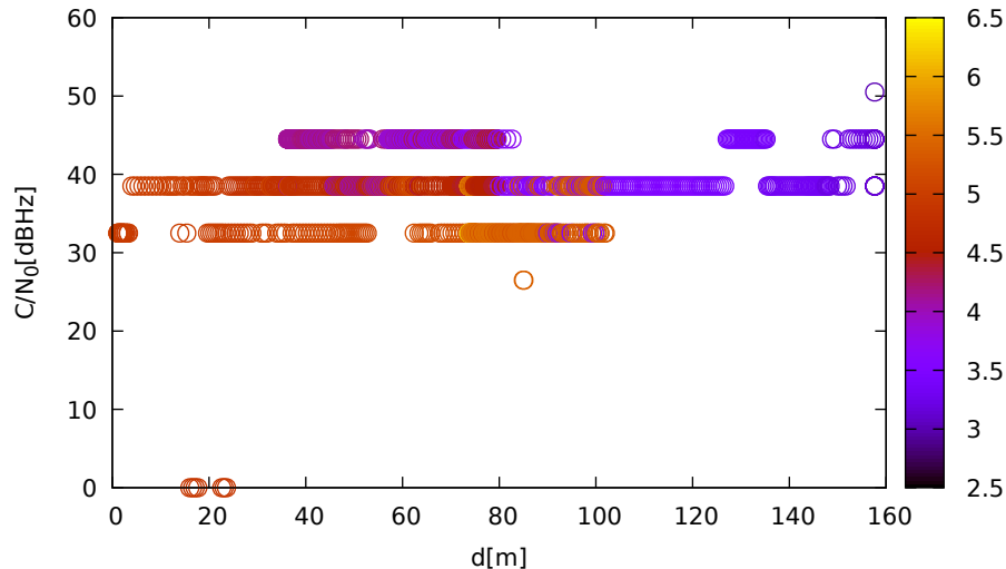
C/N 0 vs distance (LeicaGS18 at C 2 for R14 at L2)
