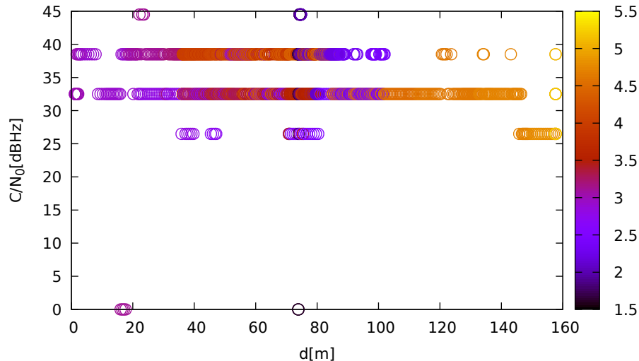
C/N 0 vs distance (LeicaGS18 at C 2 for R15 at L2)
