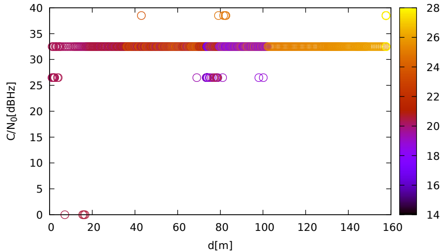
C/N 0 vs distance (LeicaGS18 at C 2 for R23 at L2)
