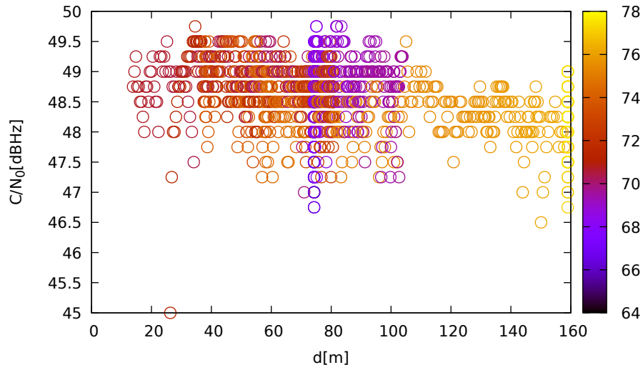
C/N 0 vs distance (TrimbleR10 at C 2 for G01 at L2)
