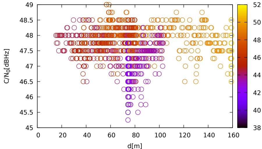
C/N 0 vs distance (TrimbleR10 at C 2 for G03 at L2)
