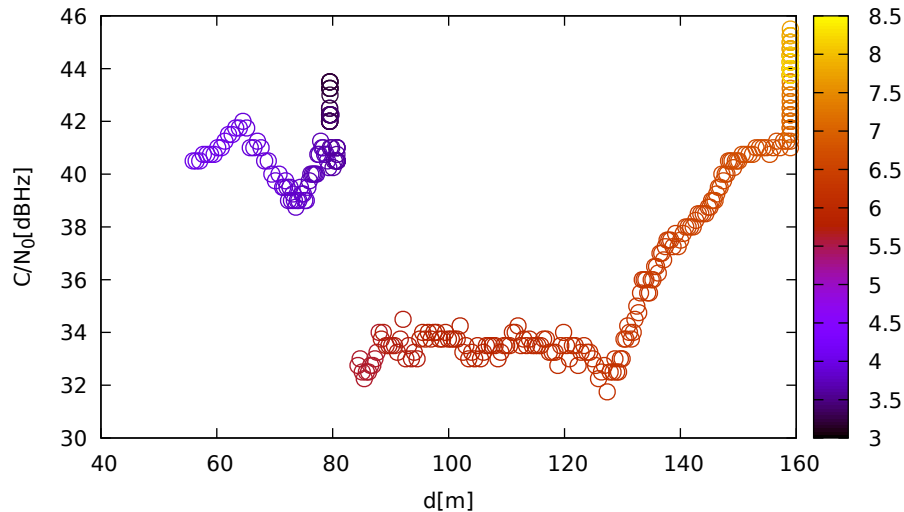
C/N 0 vs distance (TrimbleR10 at C 2 for G04 at L2)
