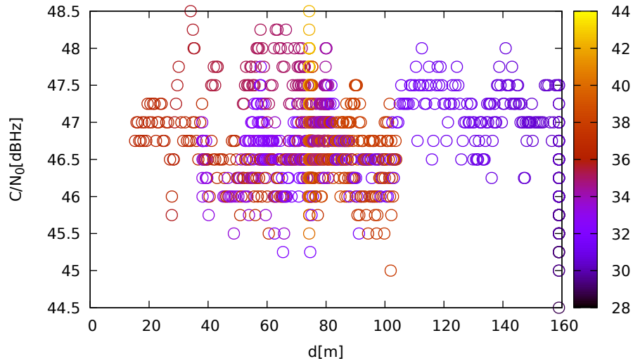
C/N 0 vs distance (TrimbleR10 at C 2 for G08 at L2)
