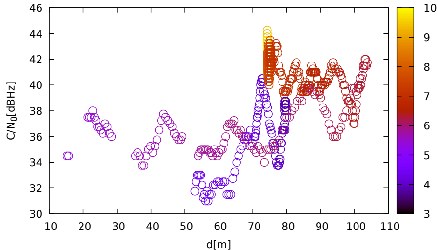
C/N 0 vs distance (TrimbleR10 at C 2 for G10 at L2)
