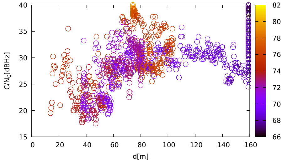
C/N 0 vs distance (TrimbleR10 at C 2 for G11 at L2)
