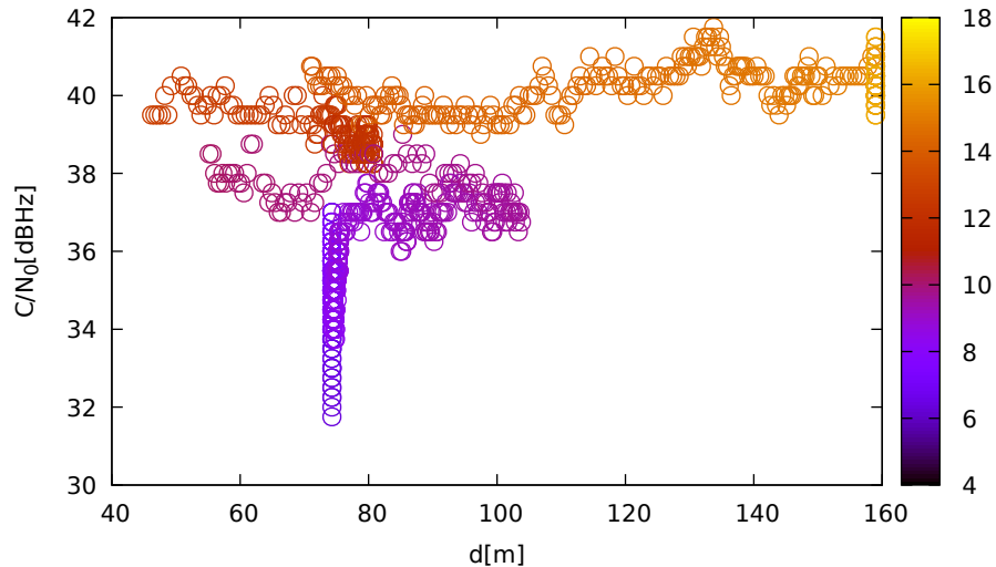
C/N 0 vs distance (TrimbleR10 at C 2 for G17 at L2)
