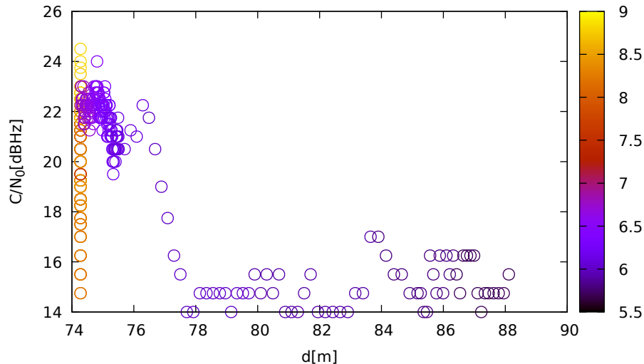
C/N 0 vs distance (TrimbleR10 at C 2 for G21 at L2)
