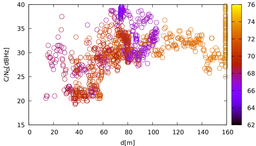
C/N 0 vs distance (TrimbleR10 at C 2 for G22 at L2)
