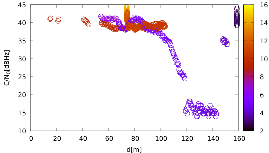
C/N 0 vs distance (TrimbleR10 at C 2 for G27 at L2)
