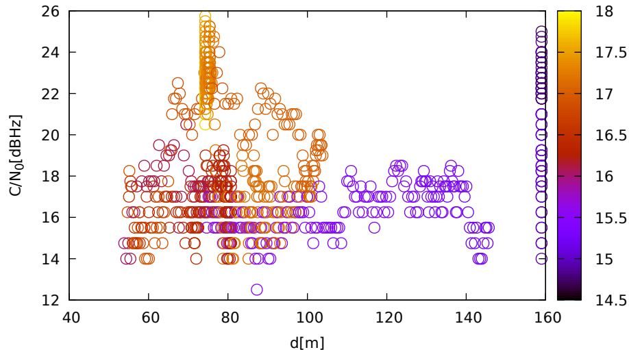
C/N 0 vs distance (TrimbleR10 at C 2 for G28 at L2)
