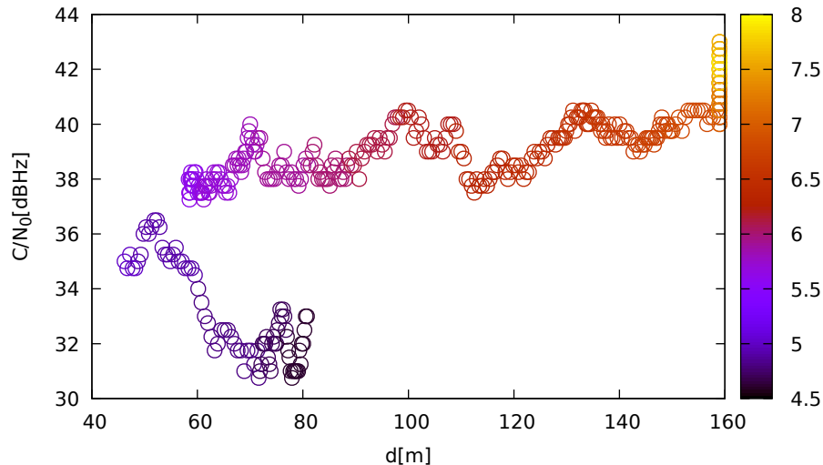
C/N 0 vs distance (TrimbleR10 at C 2 for G31 at L2)
