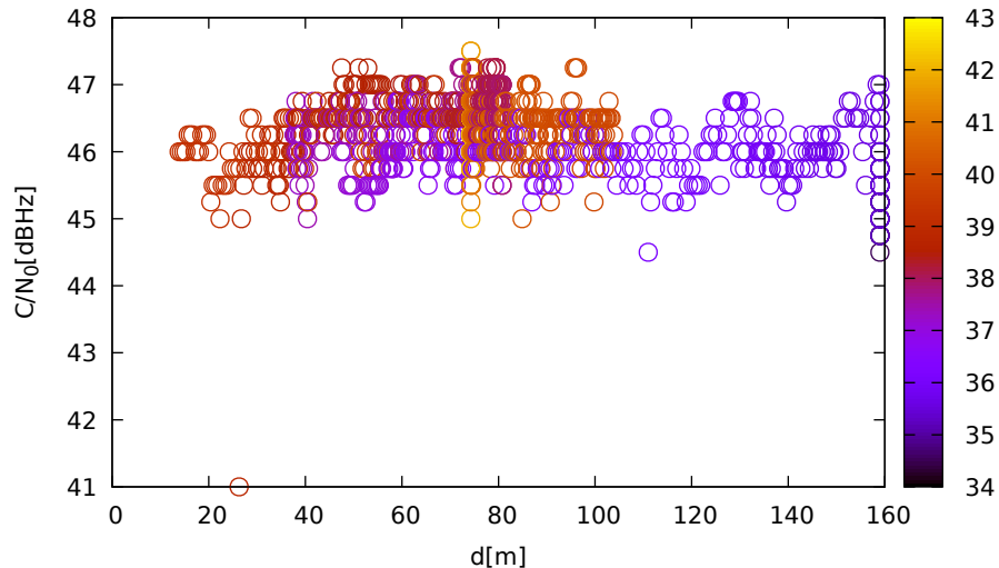
C/N 0 vs distance (TrimbleR10 at C 2 for G32 at L2)
