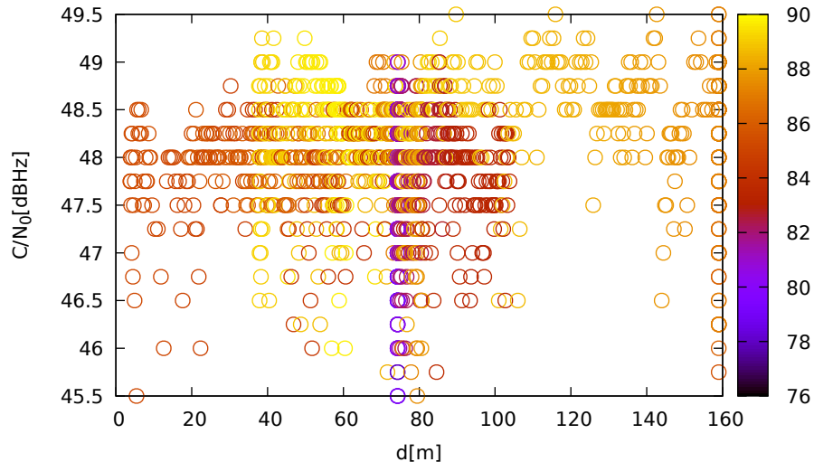
C/N 0 vs distance (TrimbleR10 at C 2 for R07 at L2)
