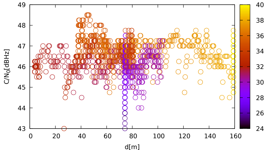
C/N 0 vs distance (TrimbleR10 at C 2 for R08 at L2)
