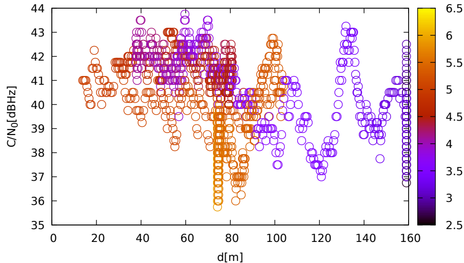
C/N 0 vs distance (TrimbleR10 at C 2 for R14 at L2)
