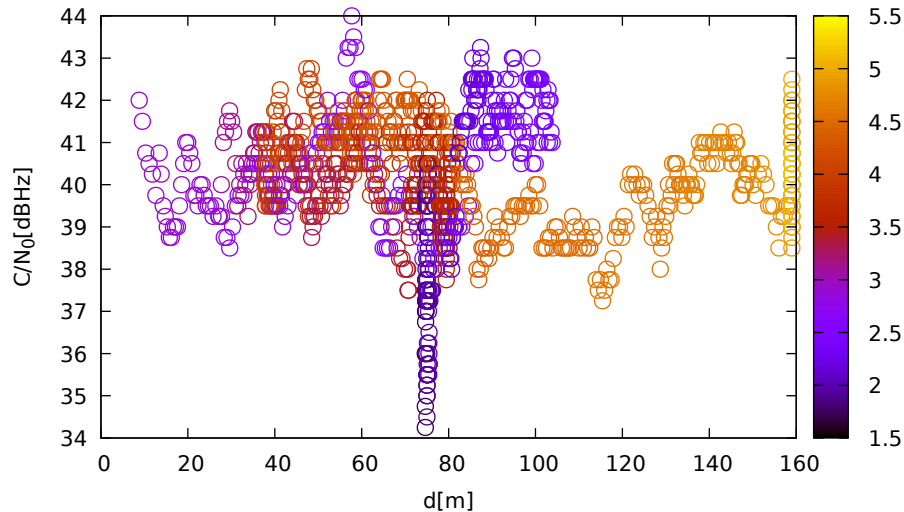
C/N 0 vs distance (TrimbleR10 at C 2 for R15 at L2)
