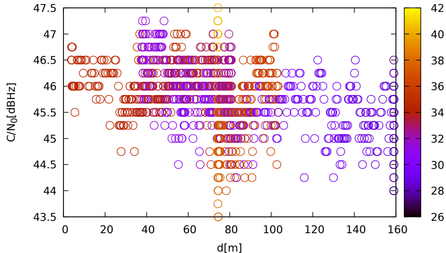
C/N 0 vs distance (TrimbleR10 at C 2 for R21 at L2)
