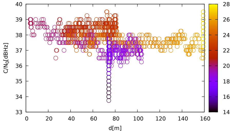
C/N 0 vs distance (TrimbleR10 at C 2 for R23 at L2)
