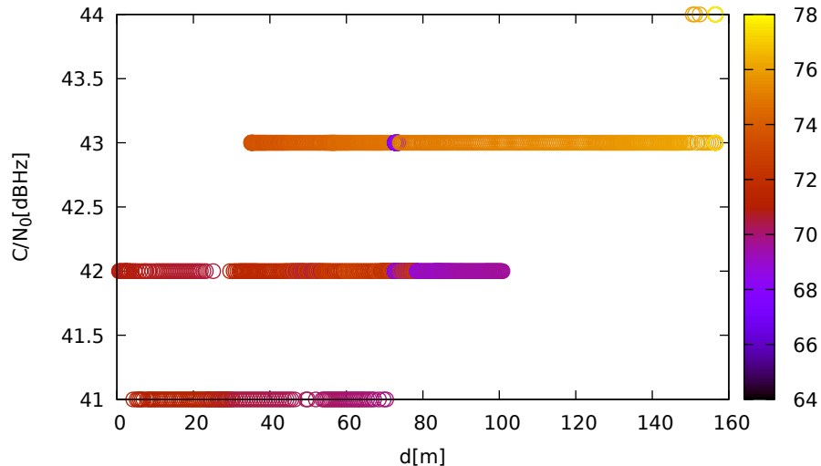
C/N 0 vs distance (ublox9 at C 2 for G01 at L2)
