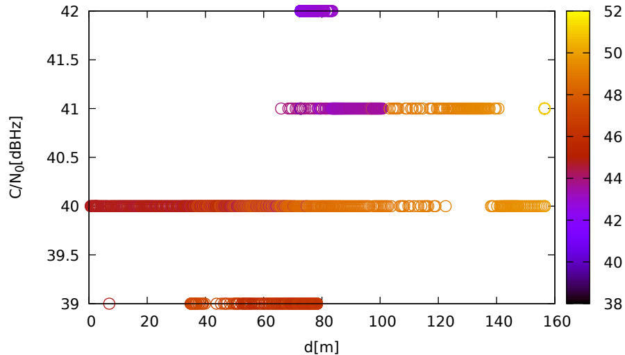
C/N 0 vs distance (ublox9 at C 2 for G03 at L2)
