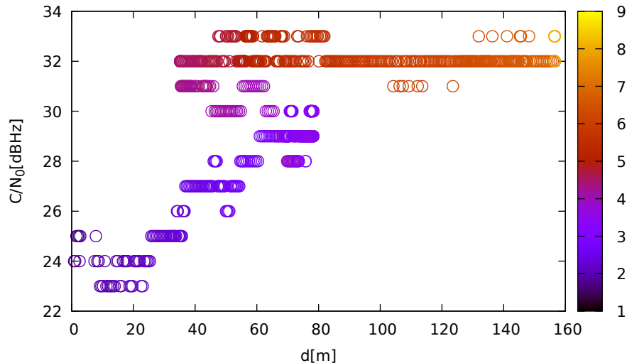
C/N 0 vs distance (ublox9 at C 2 for G04 at L2)
