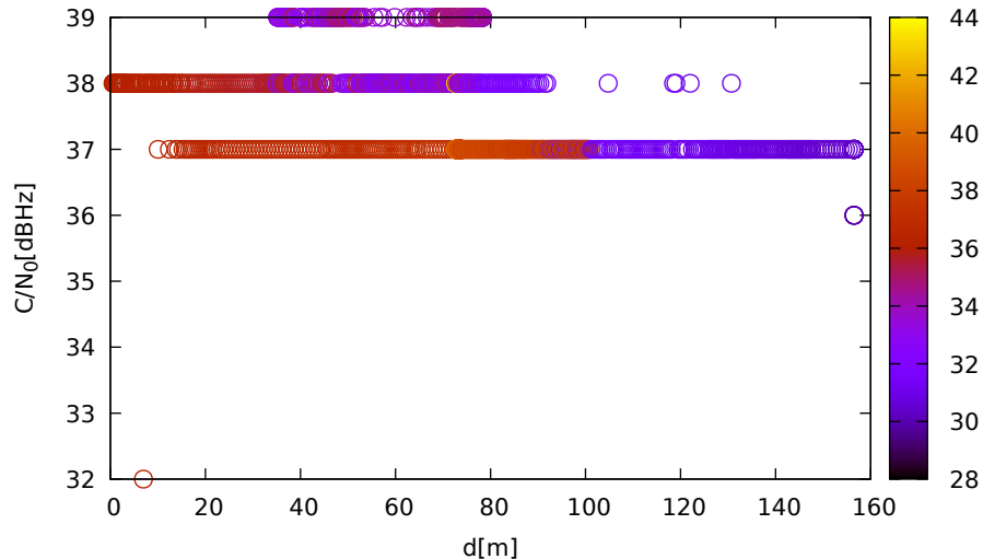
C/N 0 vs distance (ublox9 at C 2 for G08 at L2)
