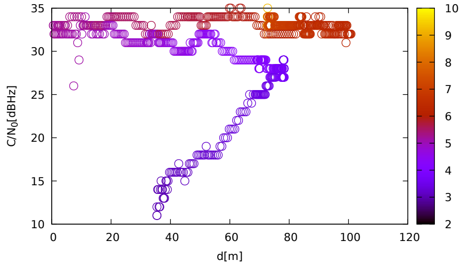
C/N 0 vs distance (ublox9 at C 2 for G10 at L2)
