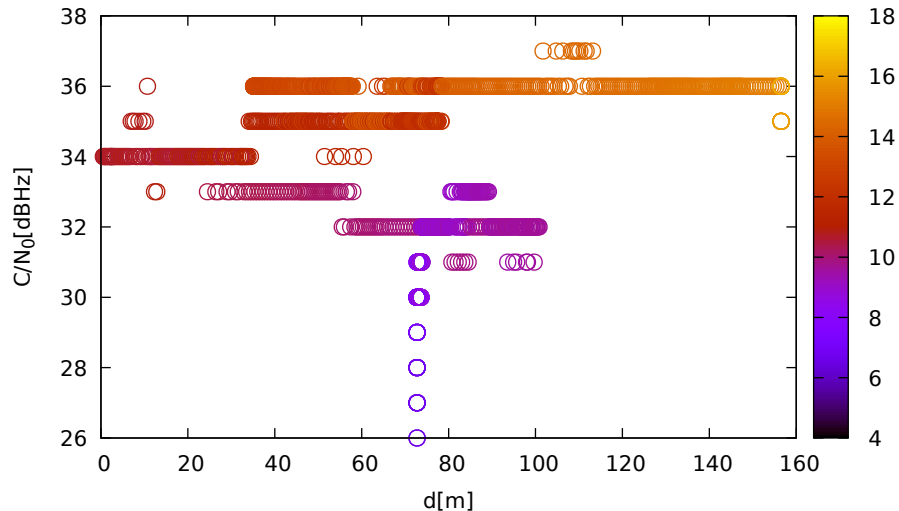
C/N 0 vs distance (ublox9 at C 2 for G17 at L2)
