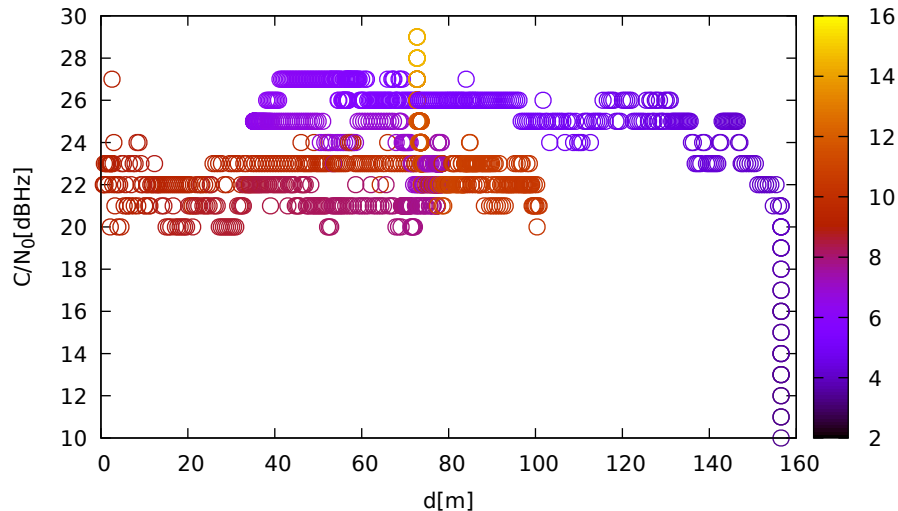
C/N 0 vs distance (ublox9 at C 2 for G27 at L2)
