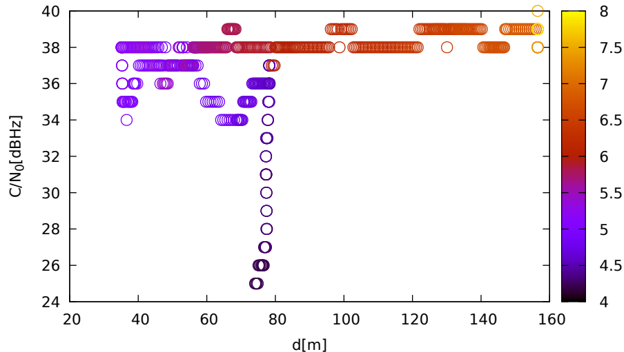
C/N 0 vs distance (ublox9 at C 2 for G31 at L2)
