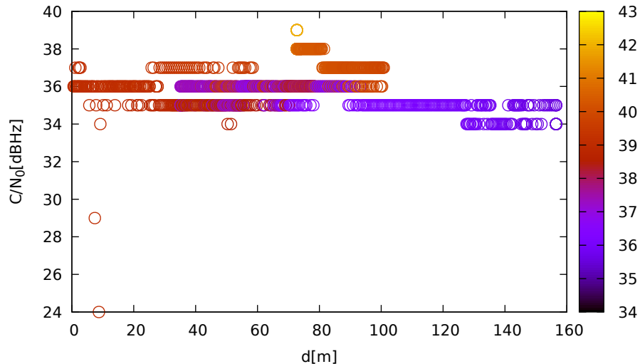
C/N 0 vs distance (ublox9 at C 2 for G32 at L2)
