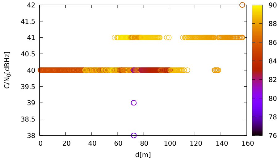
C/N 0 vs distance (ublox9 at C 2 for R07 at L2)
