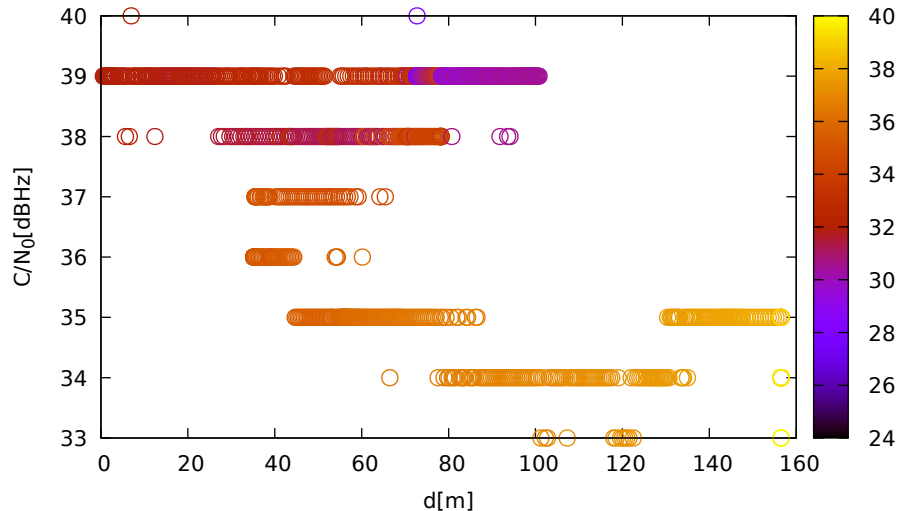
C/N 0 vs distance (ublox9 at C 2 for R08 at L2)
