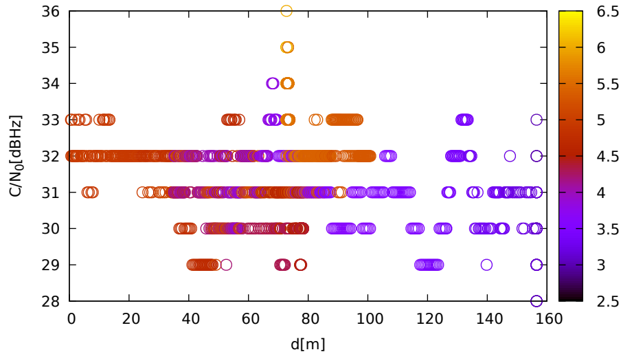
C/N 0 vs distance (ublox9 at C 2 for R14 at L2)
