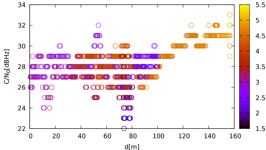
C/N 0 vs distance (ublox9 at C 2 for R15 at L2)
