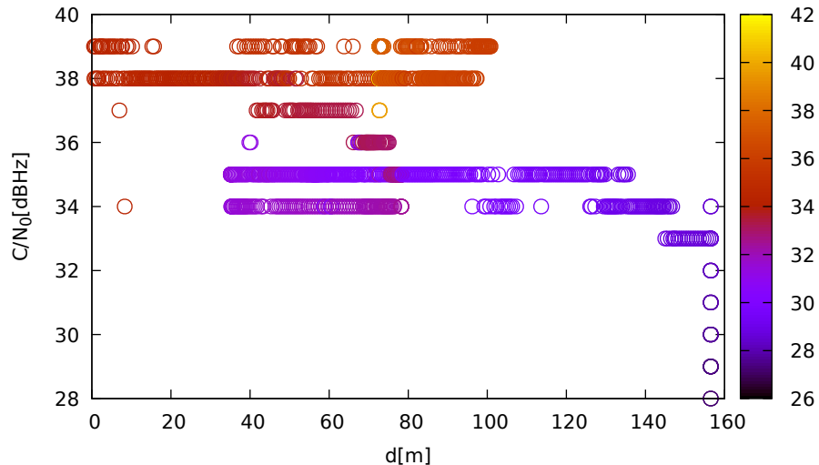
C/N 0 vs distance (ublox9 at C 2 for R21 at L2)
