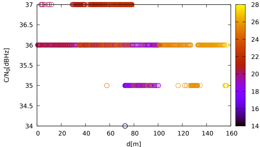
C/N 0 vs distance (ublox9 at C 2 for R23 at L2)
