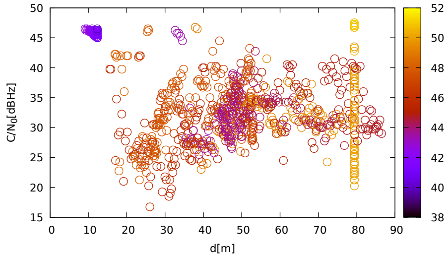
C/N 0 vs distance (JavadLSA at C 3 for G03 at L2)
