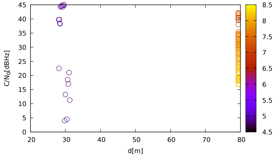
C/N 0 vs distance (JavadLSA at C 3 for G04 at L2)
