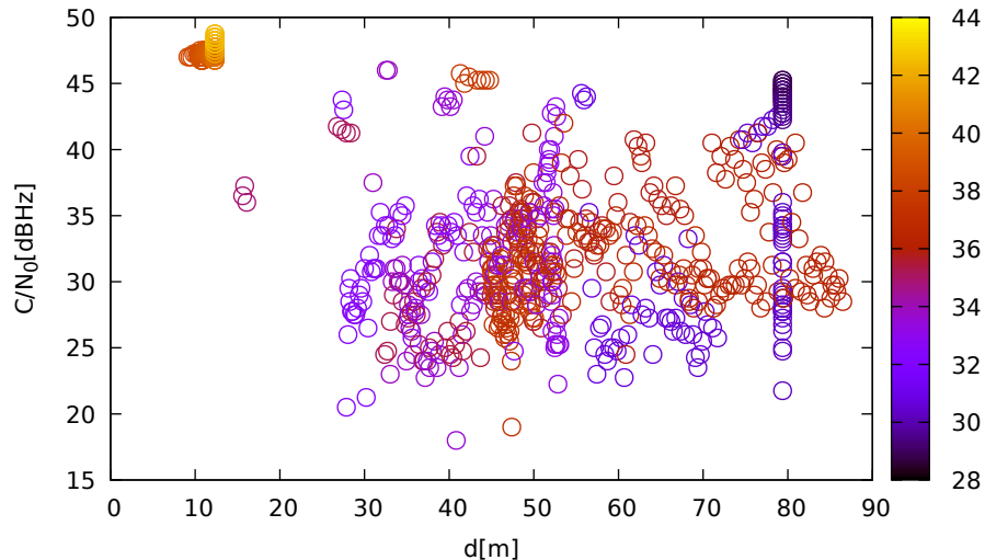
C/N 0 vs distance (JavadLSA at C 3 for G08 at L2)
