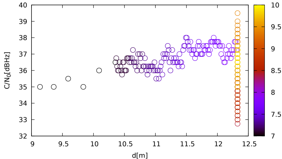
C/N 0 vs distance (JavadLSA at C 3 for G10 at L2)
