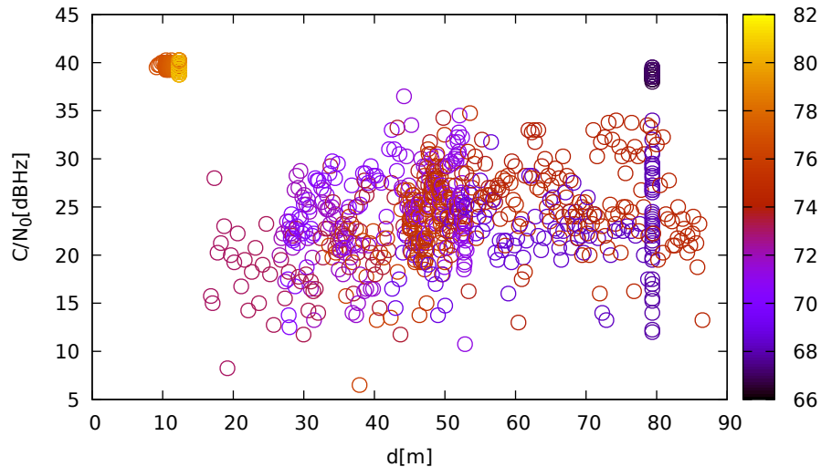
C/N 0 vs distance (JavadLSA at C 3 for G11 at L2)
