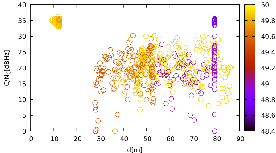
C/N 0 vs distance (JavadLSA at C 3 for G14 at L2)
