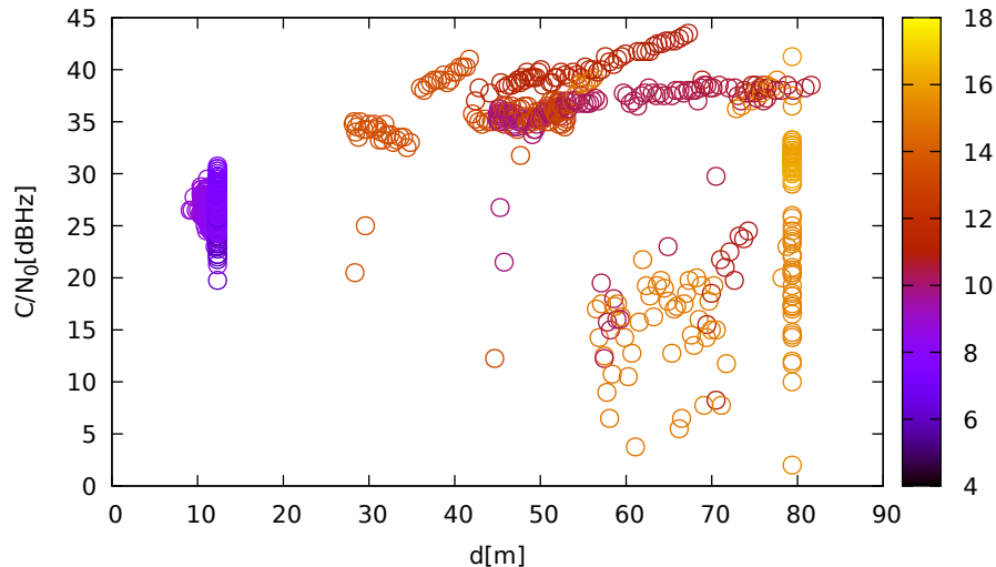
C/N 0 vs distance (JavadLSA at C 3 for G17 at L2)
